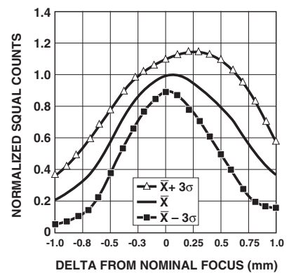
Figure 38. Typical mean squal vs. Z (white paper)
